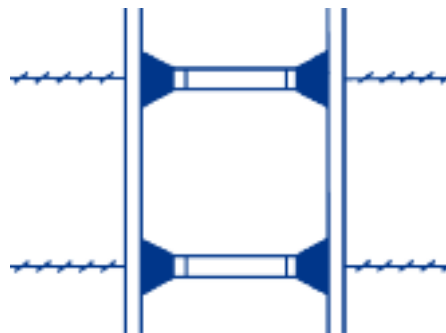
Formwork Ties
