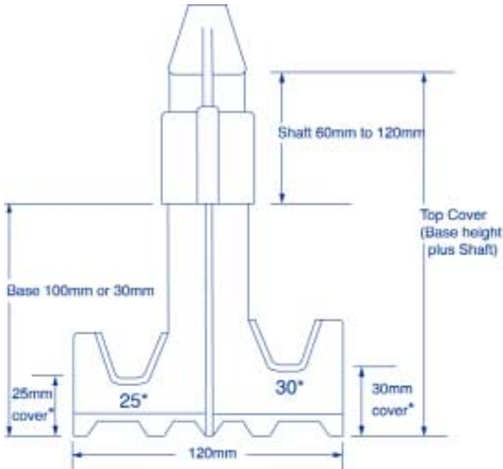
DECK CHAIR ASSEMBLED (100 mm base depicted above)
